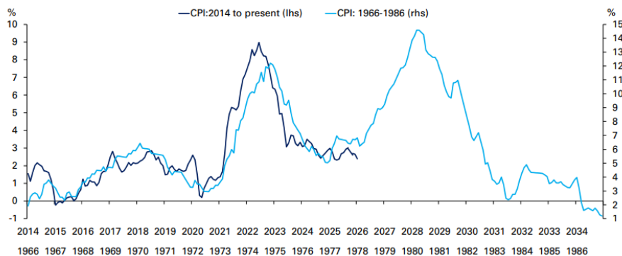
Figure 1: US Inflation: 1970s vs Today (Different Scales). The chart often gets derided but eerie that Iran now links the second shock in both cycles.
